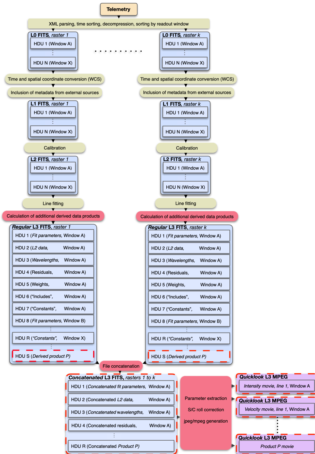
Figure 3-1 Pipeline dataflow: narrow-slit spectral-profile. Red colour signals planned processing steps and HDUs/file types that are not yet part of the pipeline. Concatenated L3 files will only be made for repeated rasters.
